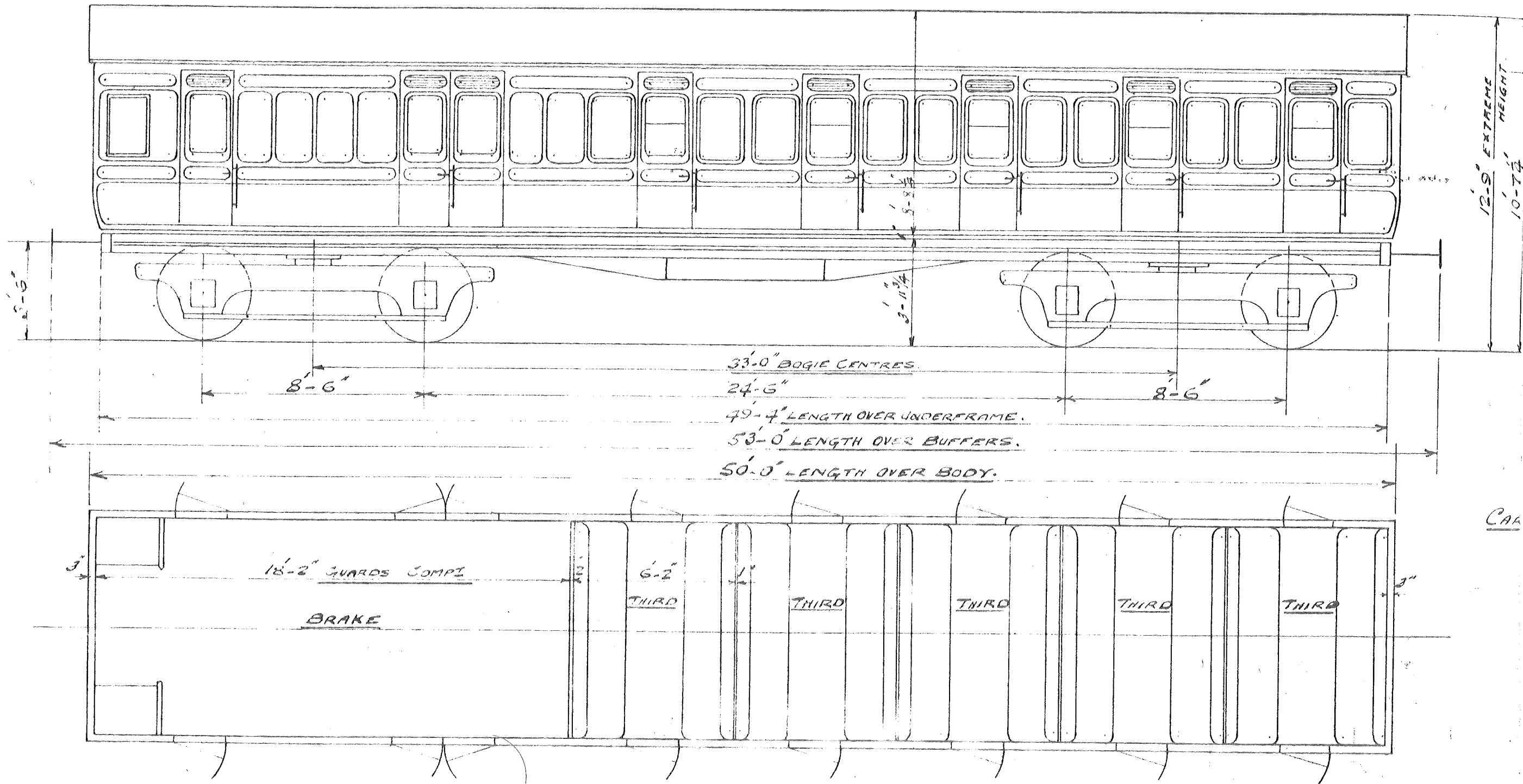
C.L.C. BOGIE THIRD CLASS AND BRAKE CARRIAGE.
